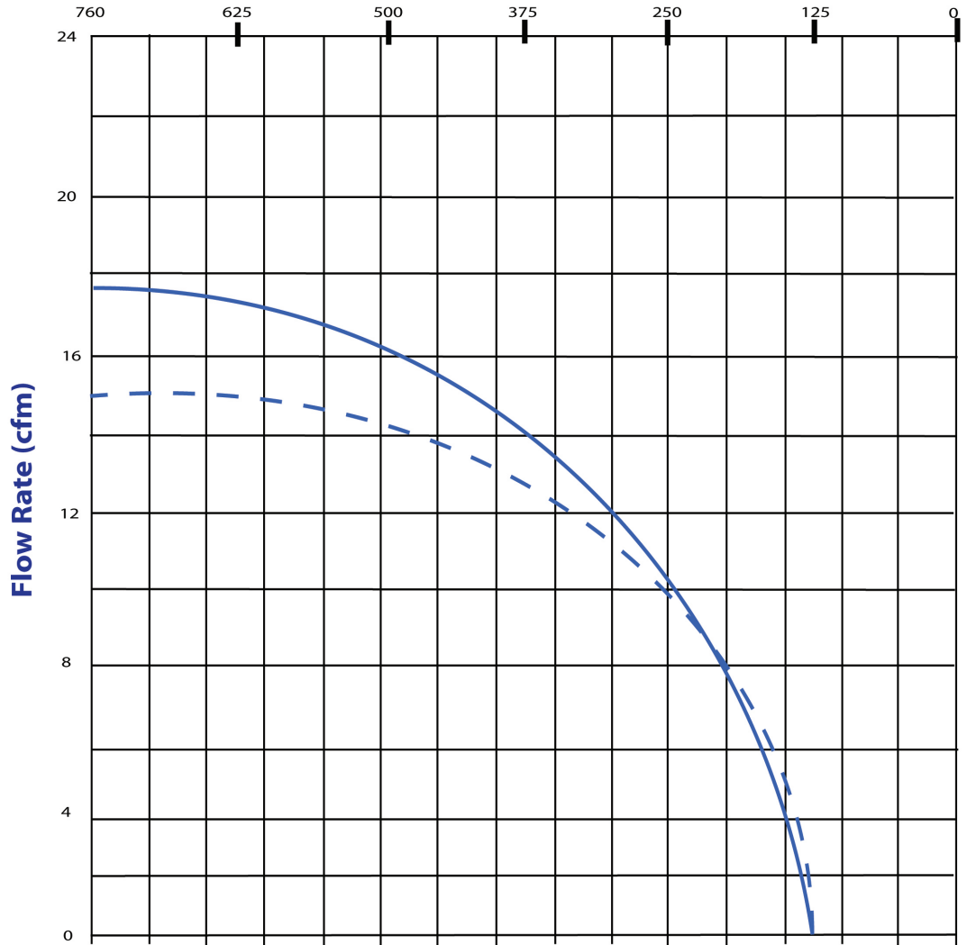
Flow Rate vs. Vacuum
